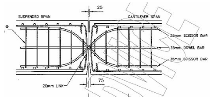
Fig. 13. Typical hinge detail showing the 2 scissor and 1 central dowel bars crossing at the center of the hinge.
